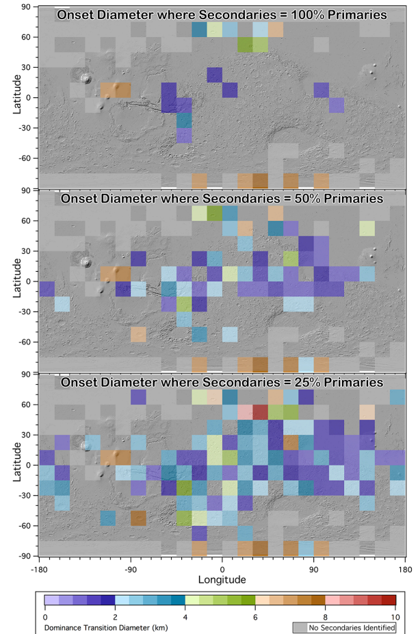
Figure 3: Several onset fractions for secondary craters in 15^\circ \times 15^\circ area bins. Grey areas are where classified secondary craters are not significant (to the stated threshold for the panel) for D \geq 1.0 km, and holes are where there were not enough craters ( \geq 50 ) for the analysis.
